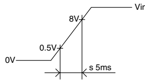
Input start-up time: 5ms or less
