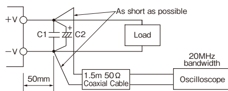
Fig.3-2 Measurement of Maximum Output Ripple & Noise Using coaxial cable
